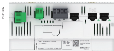
Connection points
