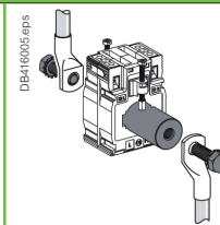
METSECT5CYL1 (aluminium)
